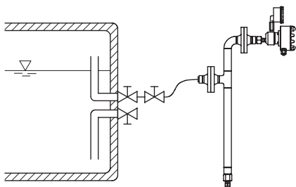
Fig. 6: Installation of the drum
