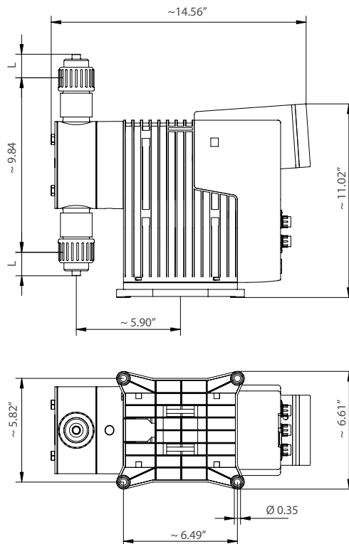
MEMDOS SMART 60 – 180 All dimensions in inches
